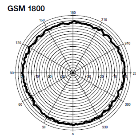
Radiation Pattern (900 / 1800MHz)
