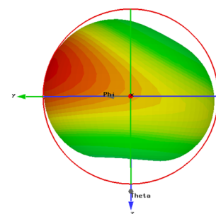
Simulated Radiating Pattern Directivity @ 700MHz
