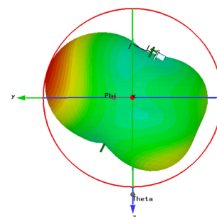
Simulated Radiating Pattern Directivity @ 1900MHz
