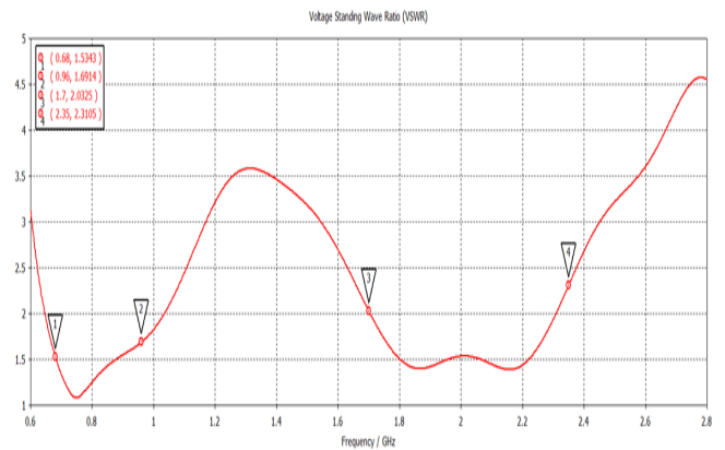
Simulated VSWR Chart
